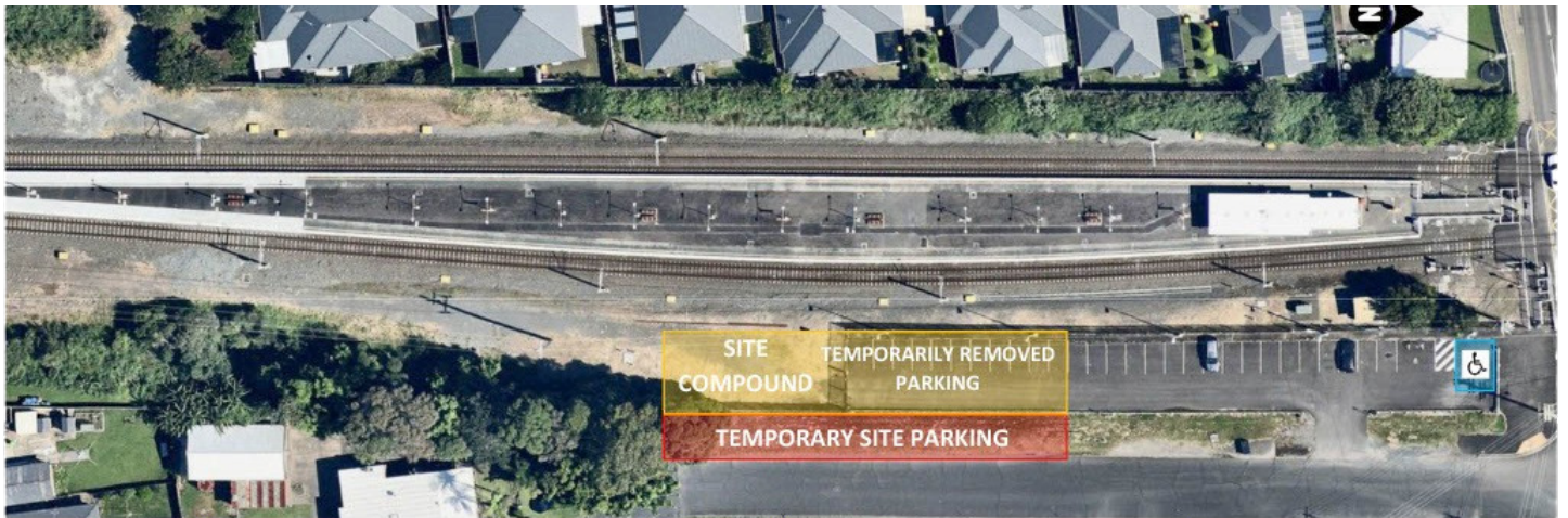
Pictured: site compound and commuter carpark plan.
