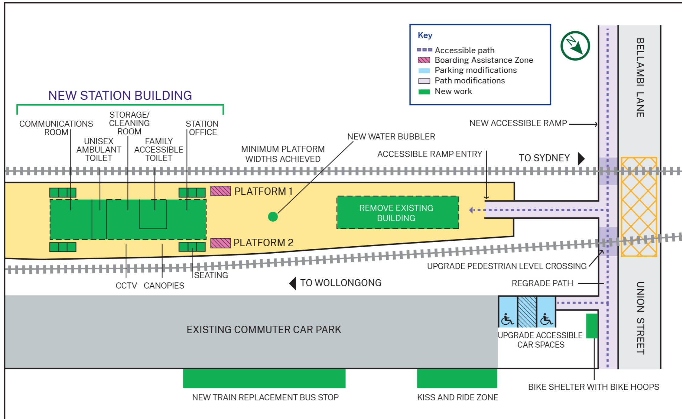
Pictured: Bellambi Station upgrade key features plan
