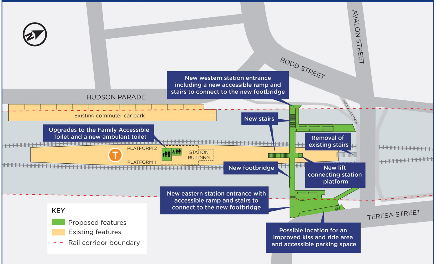
Key features of the proposed Birrong Station upgrade.
